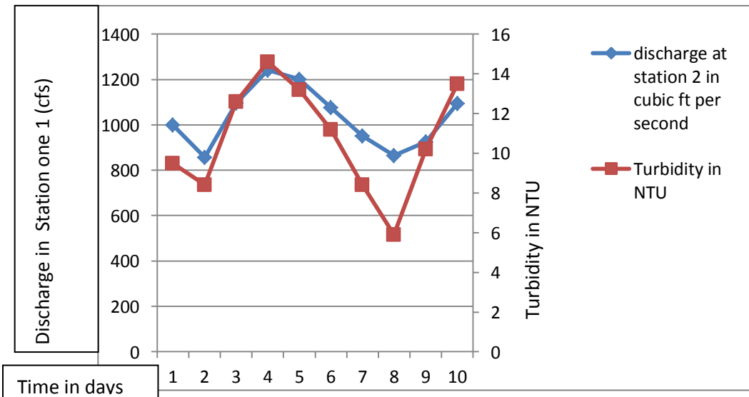
Discharge at Station 2 vs. Turbidity at Buoy
