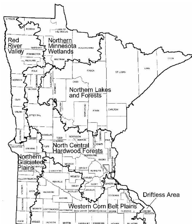
Figure 1: Minnesota Ecoregions
