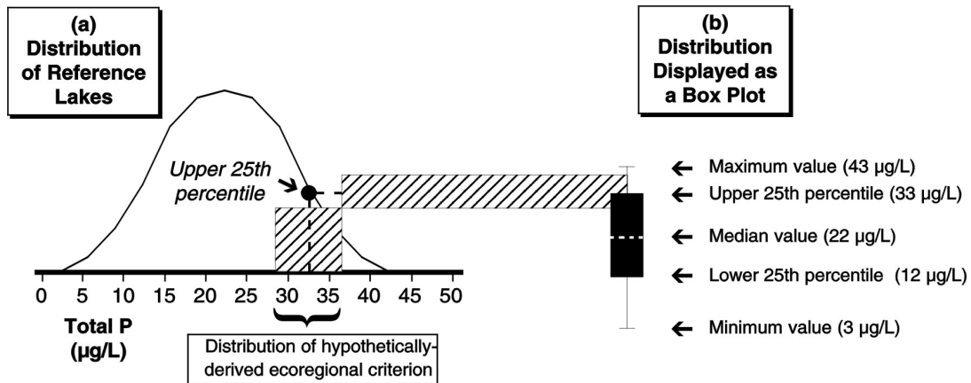
Figure 7.1. Development of a hypothetical ecoregional reference condition for TP from an ecoregion data set of reference lakes.
